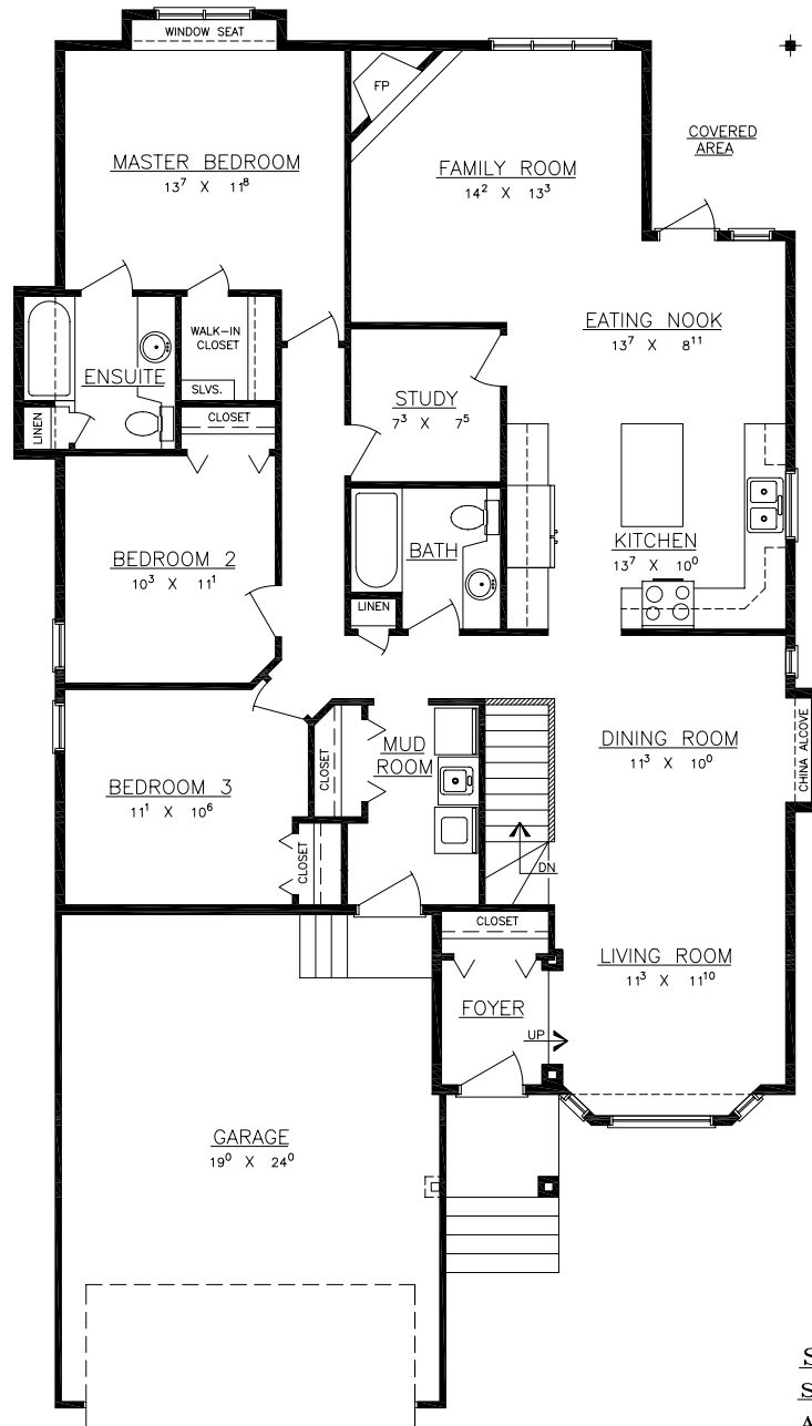
FLOOR PLAN
